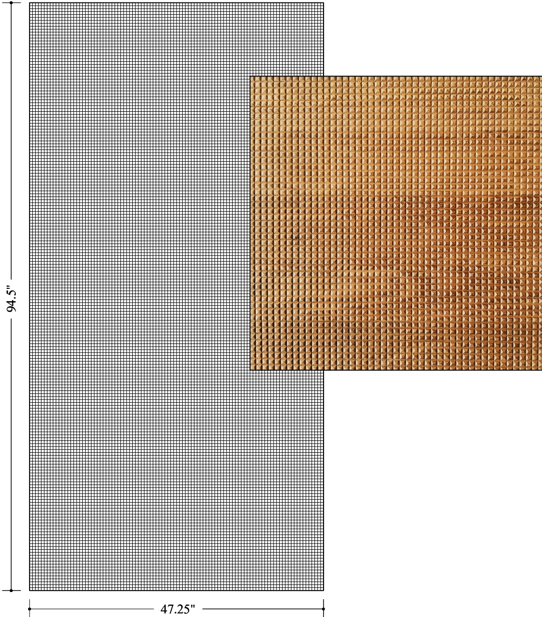
WPFSN208 (scale: 3/4" = 1'-0")
