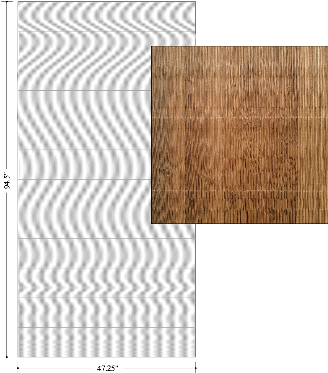
WPFSN206 (scale: 3/4" = 1'-0")
