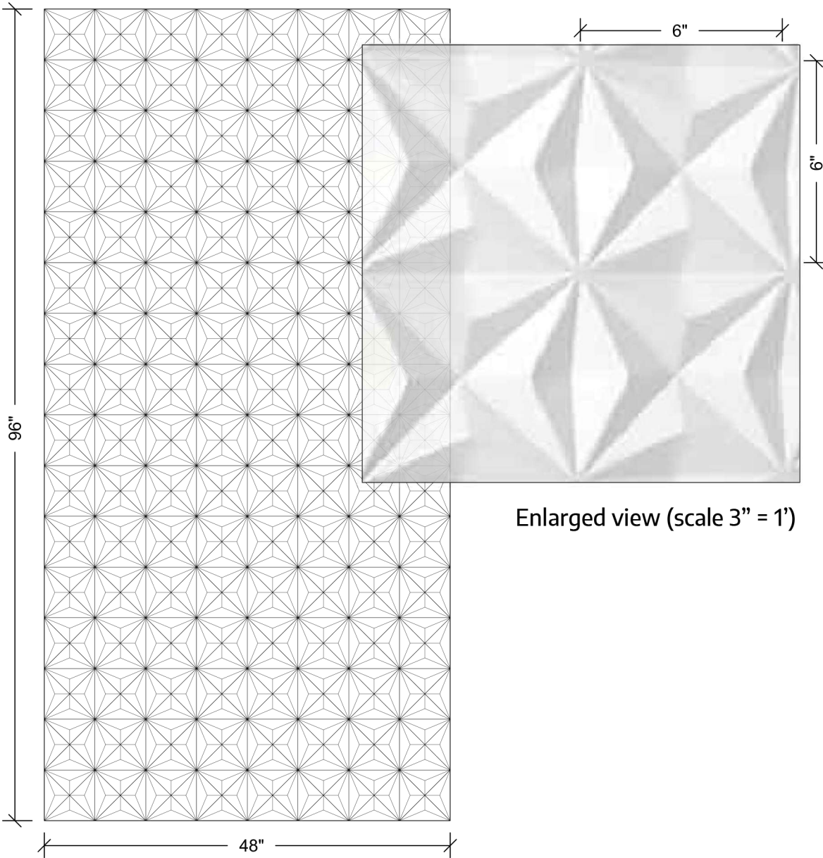
WPMAS012 (scale 3/4" = 1')
