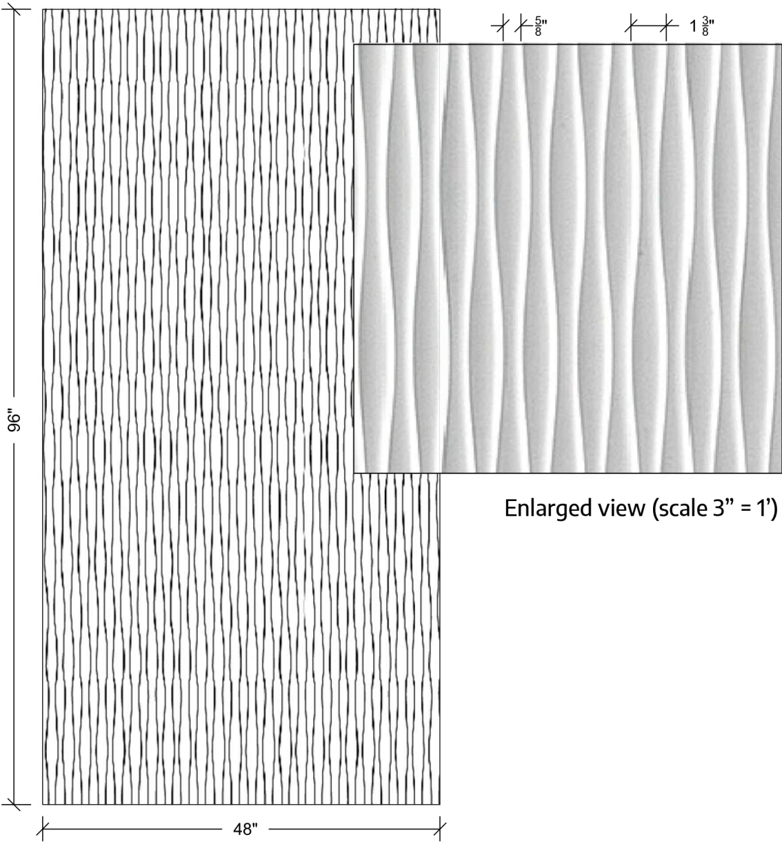
WPMAS003 (scale 3/4" = 1')
